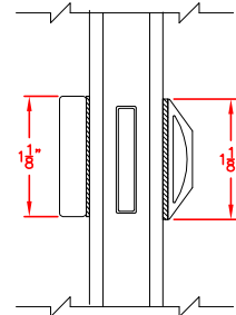
1-1/8" SQUARE SIMULATED DIVIDED LITE
