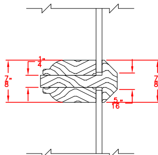
SINGLE GLAZED TDL 7/8"
