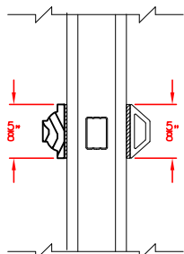
5/8" SIMULATED DIVIDED LITE
