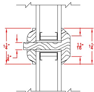
INSULATED GLASS TDL 1-1/4"
