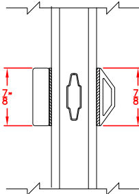
7/8" SQUARE SIMULATED DIVIDED LITE
