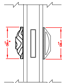
1-1/8" SIMULATED DIVIDED LITE
