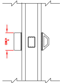
5/8" SQUARE SIMULATED DIVIDED LITE
