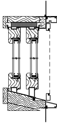
Clad Glider Vertical Section
