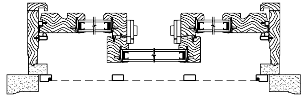
Primed Triple Picture Horizontal Section
