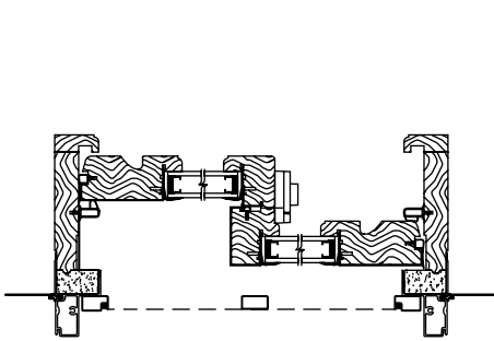
Clad Glider Horizontal Section
