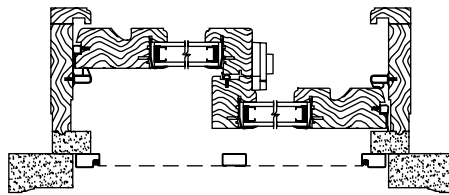
Primed Glider Horizontal Section
