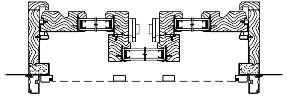
Clad Triple Picture Horizontal Section
