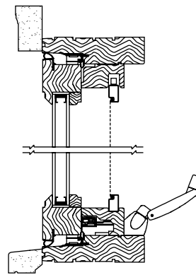
Primed Vertical Section
