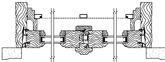
Primed Horizontal Section
