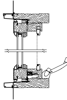
Clad Vertical Section
