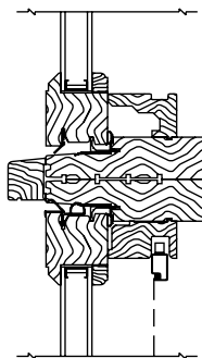
Primed Horizontal Mull Picture Vertical Section
