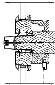
W-V Horizontal Mull Vertical Section
