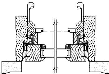
Primed Horizontal Section
