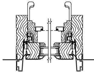
W-V Horizontal Section
