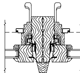
Primed Vertical Mull Horizontal Section
