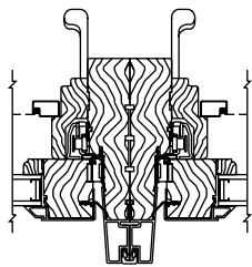
W-V Vertical Mull Horizontal Section
