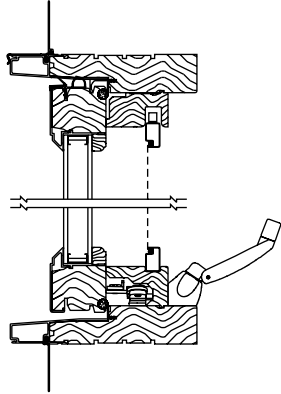
Clad Vertical Section
