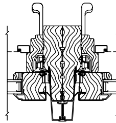
Clad Vertical Mull Horizontal Section
