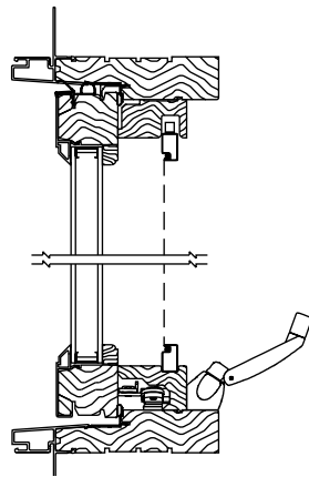
W-V Vertical Section
